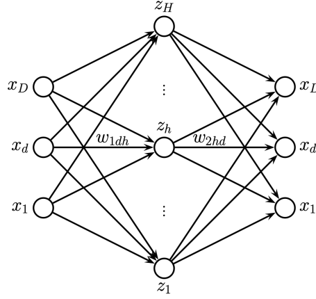
Figure 1: An autoencoder with one hidden layer MLP
